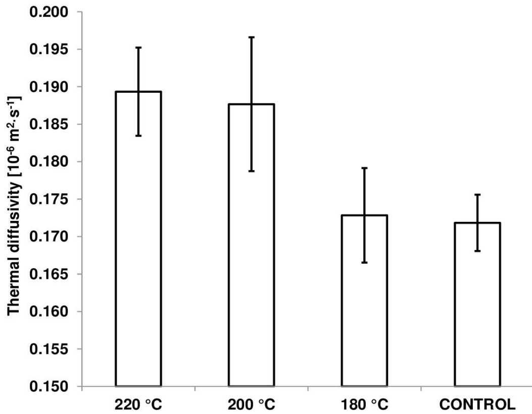
Fig. S3 - Mean values and standard deviation of thermal diffusivity.
