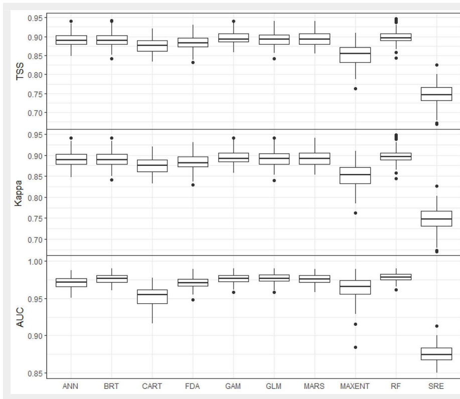
Fig. 2 - Adjustment values obtained for 10 different distribution models in Andalusia, including Artificial Neural Networks (ANN), Boosted Regression Trees (BRT), Classification and Regression Trees (CART), Flexible Discriminate Analysis (FDA), Generalized Additive Models (GAM), Generalized Linear Models (GLM), Multivariate Adaptive Regression Splines (MARS), Maximum Entropy (MaxEnt), Random Forest (RF), and Surface Range Envelop (SRE).
