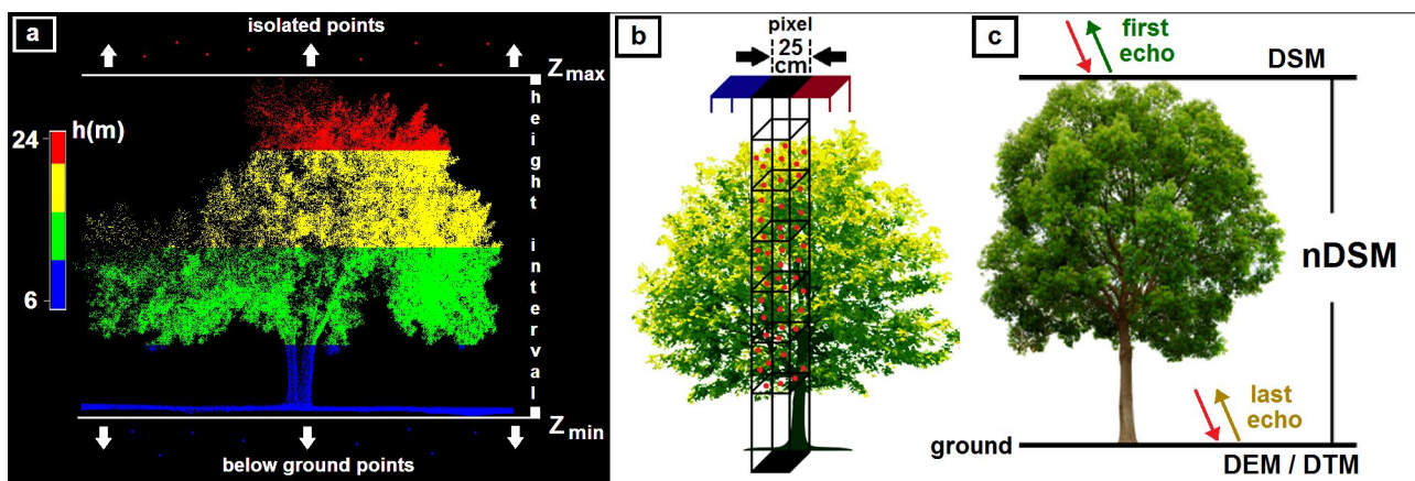
Fig. S1 - (a) Filtering of blunders, (b) elevation variety trouble in same pixel, (c) nDSM basic principle.
