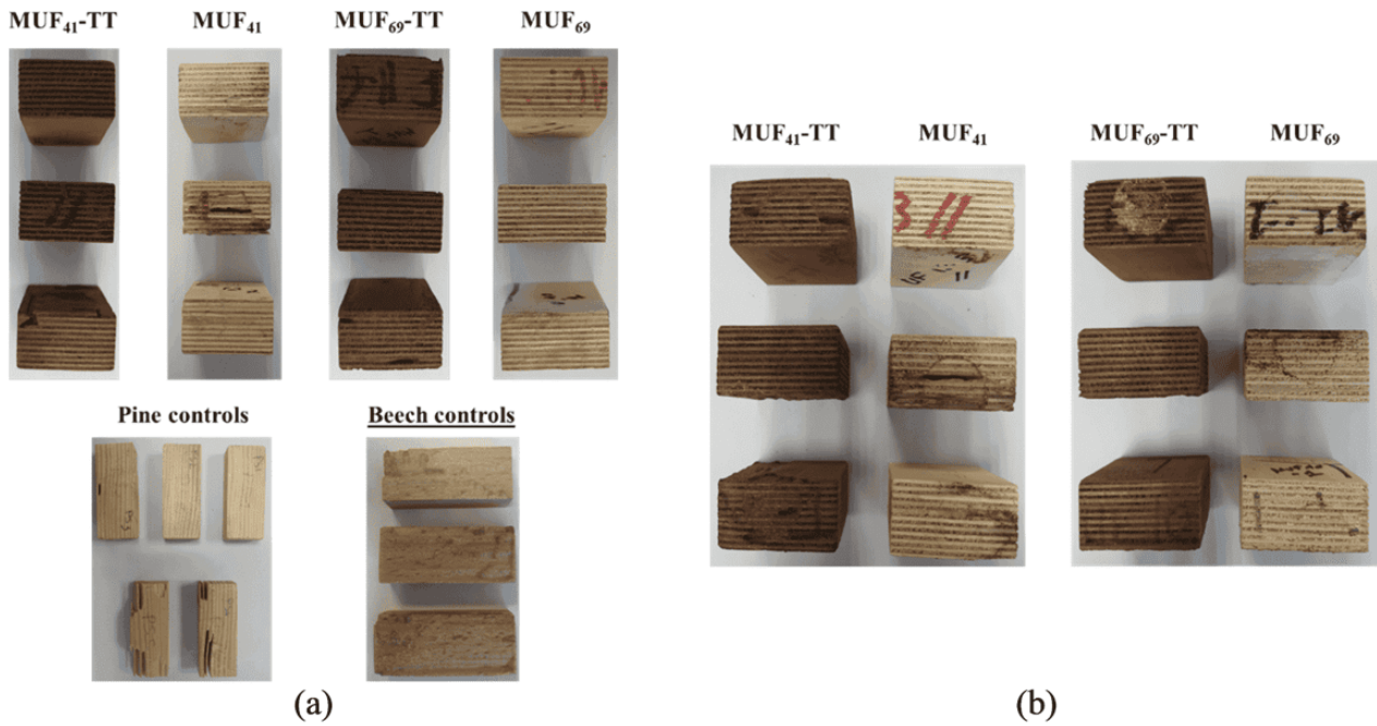
Fig. S2 - Visual appearances of plywood samples and control samples after (a) non-choice and choice (b) termite resistance test.
