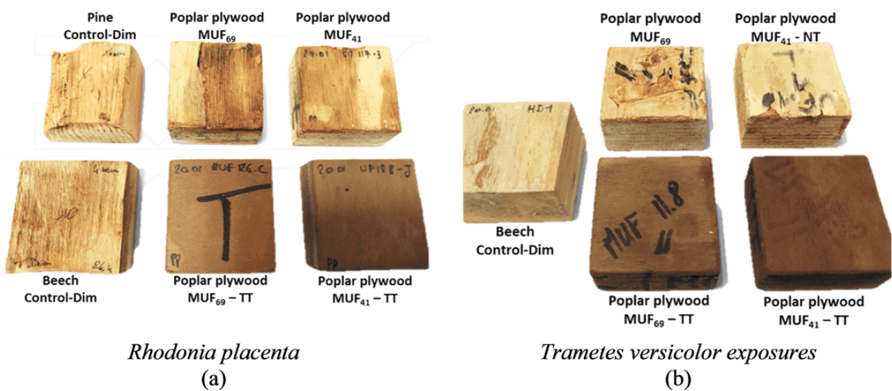
Fig. S1 - Visual aspect of the Pine Control-Dim, Beech Control-Dim, MUF69 non-treated (MUF69) and thermally treated poplar panels (MUF69-TT) and MUF41 non-treated (MUF41) and thermally treated poplar panel (MUF41-TT) samples, after 16 weeks of (a) Rhodonía placenta and (b) Trametes versicolor exposures.
