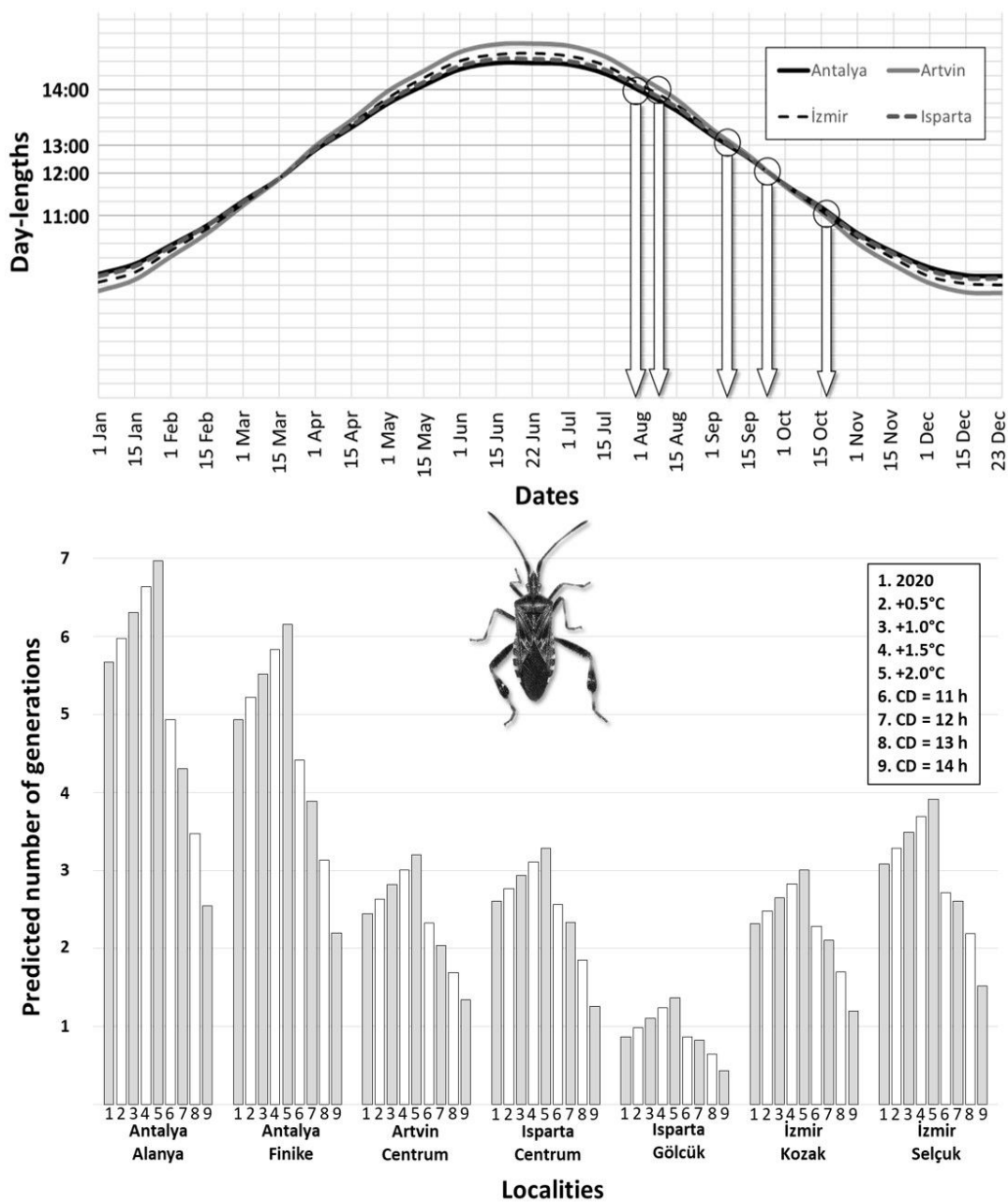
Fig. S1 - Number of generations under different temperature and critical day-length (CD) scenarios for the induction of reproductive diapause in Leptoglossus occidentalis adults in Turkey. The graphic above shows the different critical day-lengths for diapause induction and the graphic below shows the possible number of generations.
