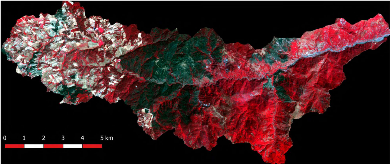
Fig. S2 - SENTINEL-2, Level 1-C image. Representation of the band set=8-4-3.
