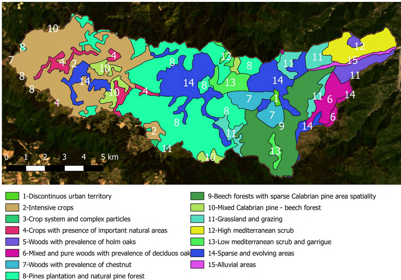
Fig. S1 - Soil use map (CLC-IV level).
