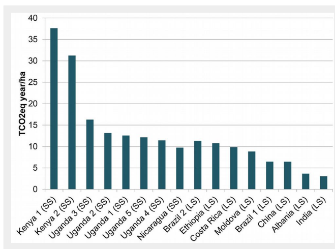
Fig. 7 - Emission reductions per hectare per year in the Italian participated CDM registered forest projects, according to the statements in the PDDs. (LS): Large Scale; (SS): small Scale .
