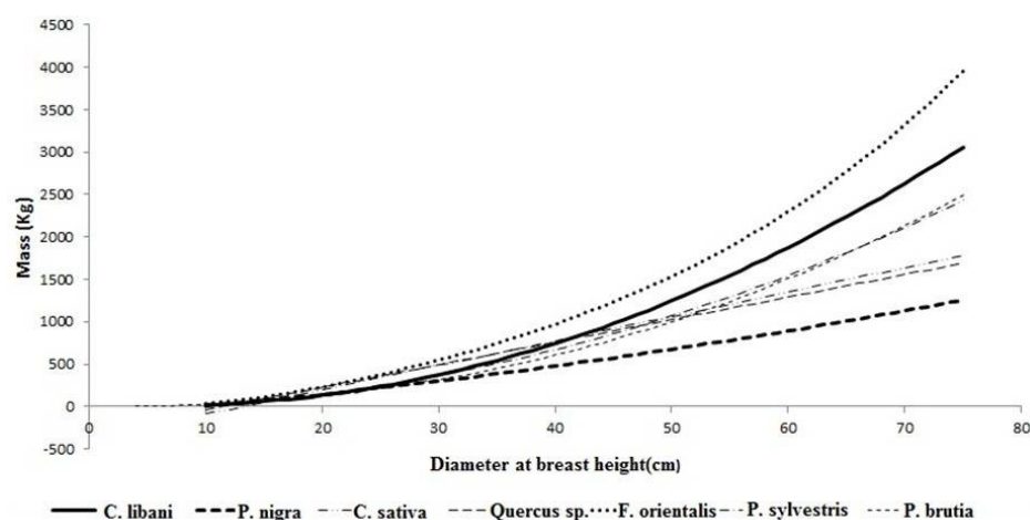
Fig. 3 - Biomass changes according to diameter at breast height in single trees according to species.
