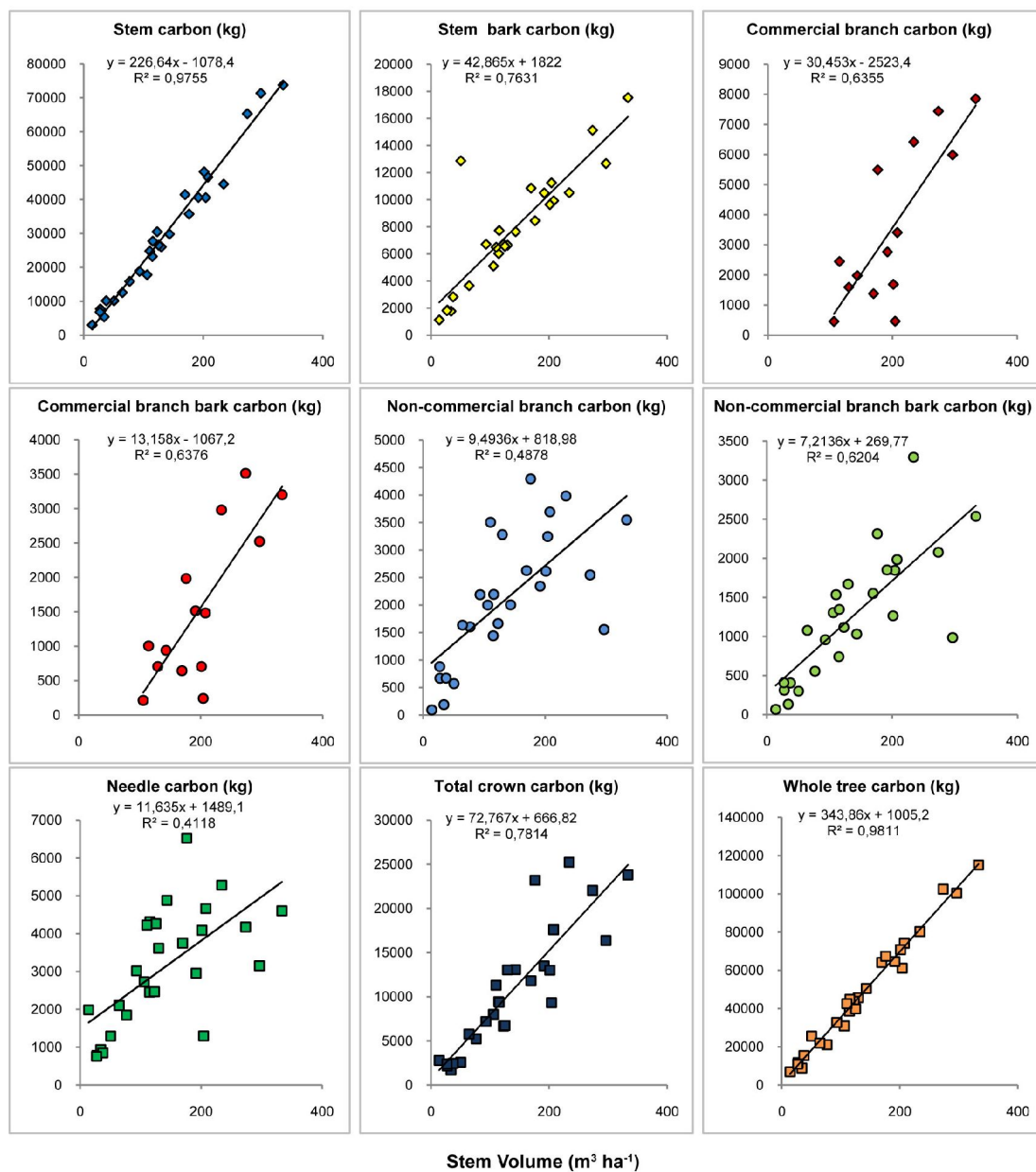
Fig. 2 - Relations between standing stem volume (m 3 ) and tree components.
