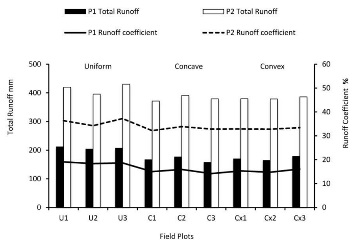
Fig. 3 - Total runoff and mean runoff coefficient on the uniform (U), concave (C), and convex (Cx) plots.
